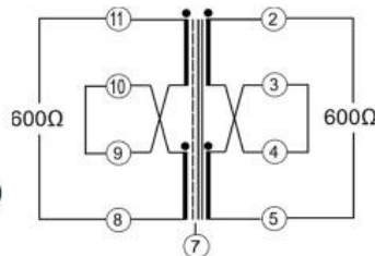
Terminal Connection
