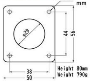
Outline Drawing
