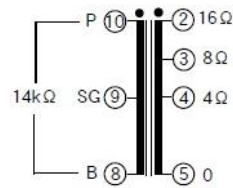
Terminal Connection
