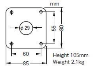
Outline Drawing
